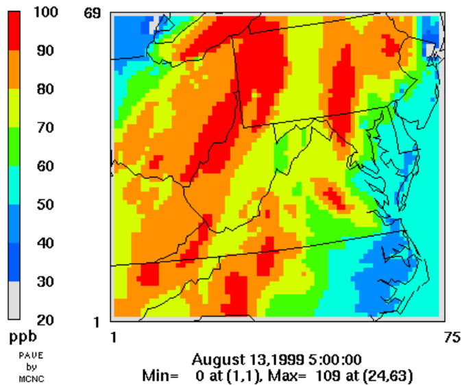
Figure 5-5. CAMx predicted 8-hour daily maximum ozone concentrations
