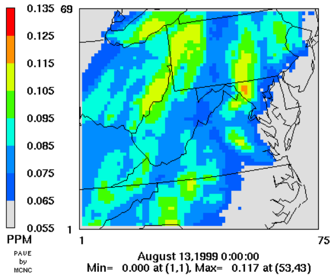
Figure 5-4. CAMx predicted 1-hour daily maximum ozone concentrations
