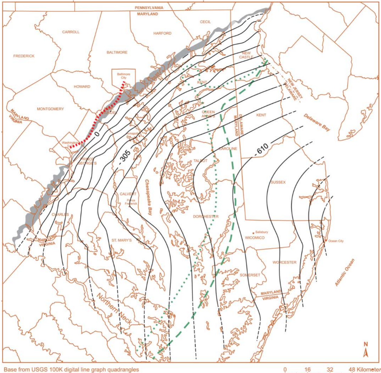
Figure D.7-8: Patapsco Aquifer in Relation to the SCMAGLEV Alignment
