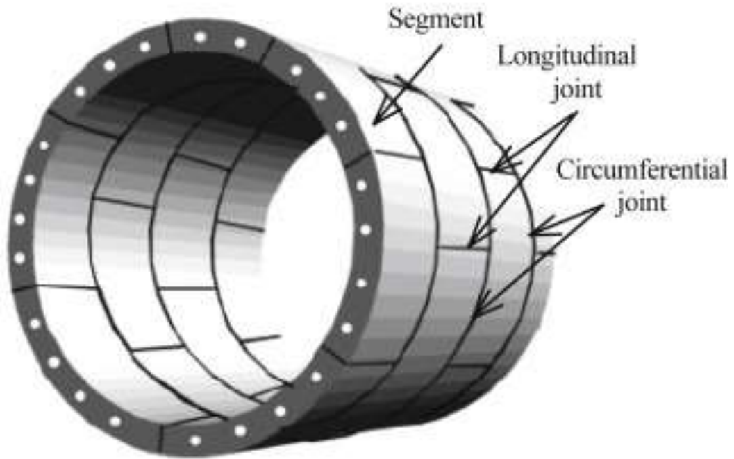
Figure 6. Typical Precast Concrete Segmental Lining (Courtesy of Herrenknecht)
