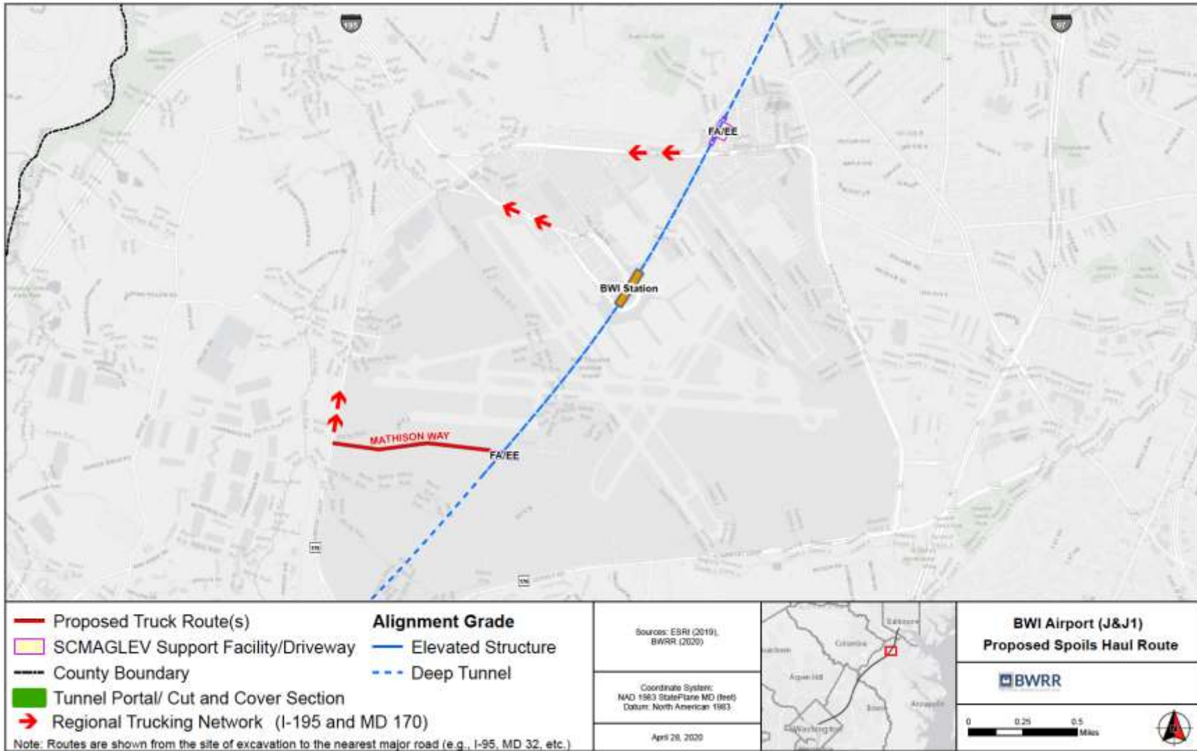
Figure 35 Proposed Haul Route for BWI Airport (Alignment Alternative J & J1)
