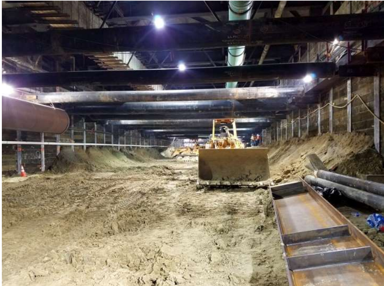
Figure 8. Typical soldier pile and lagging system (Wilshire/La Brea Station, Los Angeles, CA)
