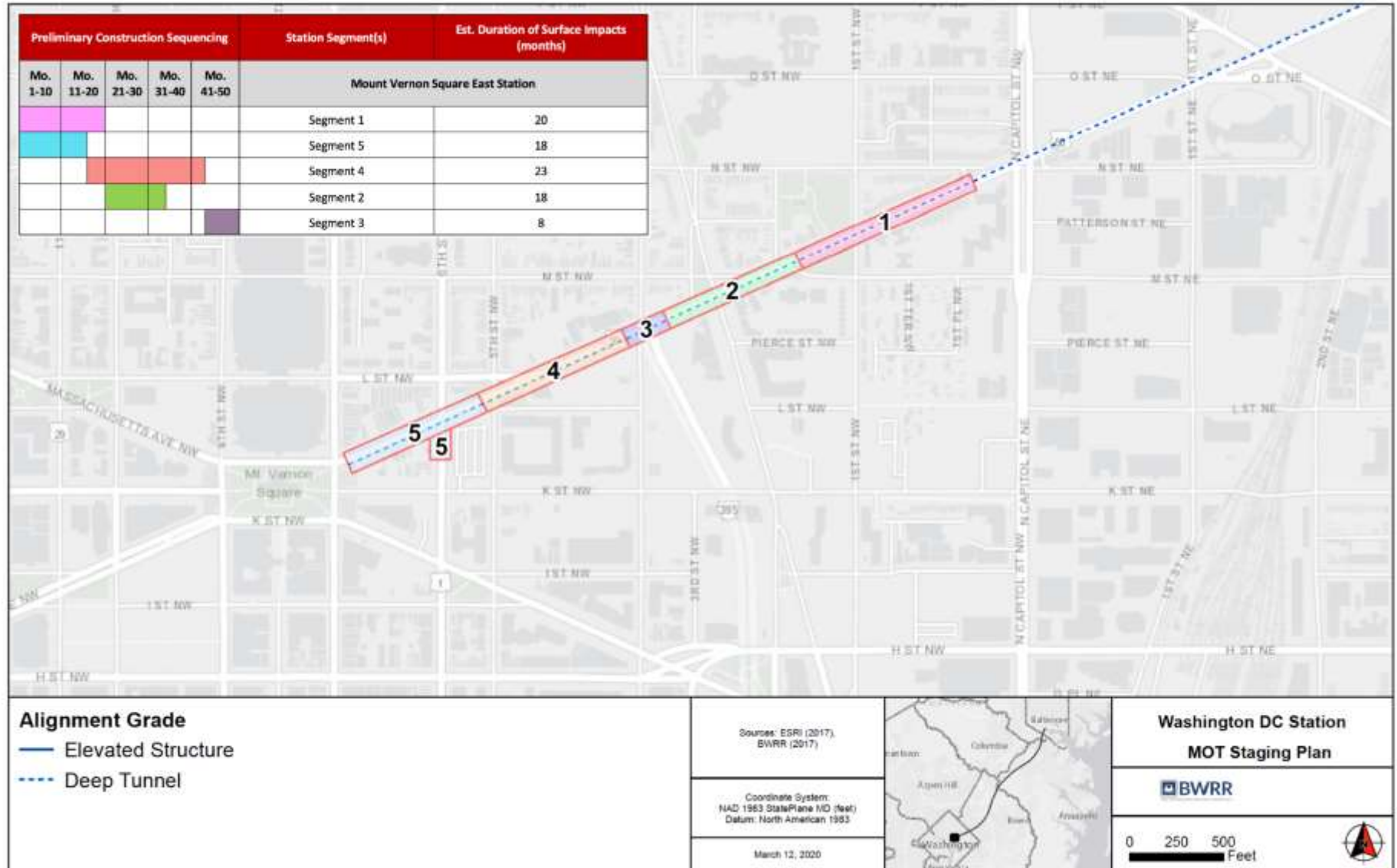
Figure 22. Construction Staging Segments for Mount Vernon Square East Station
