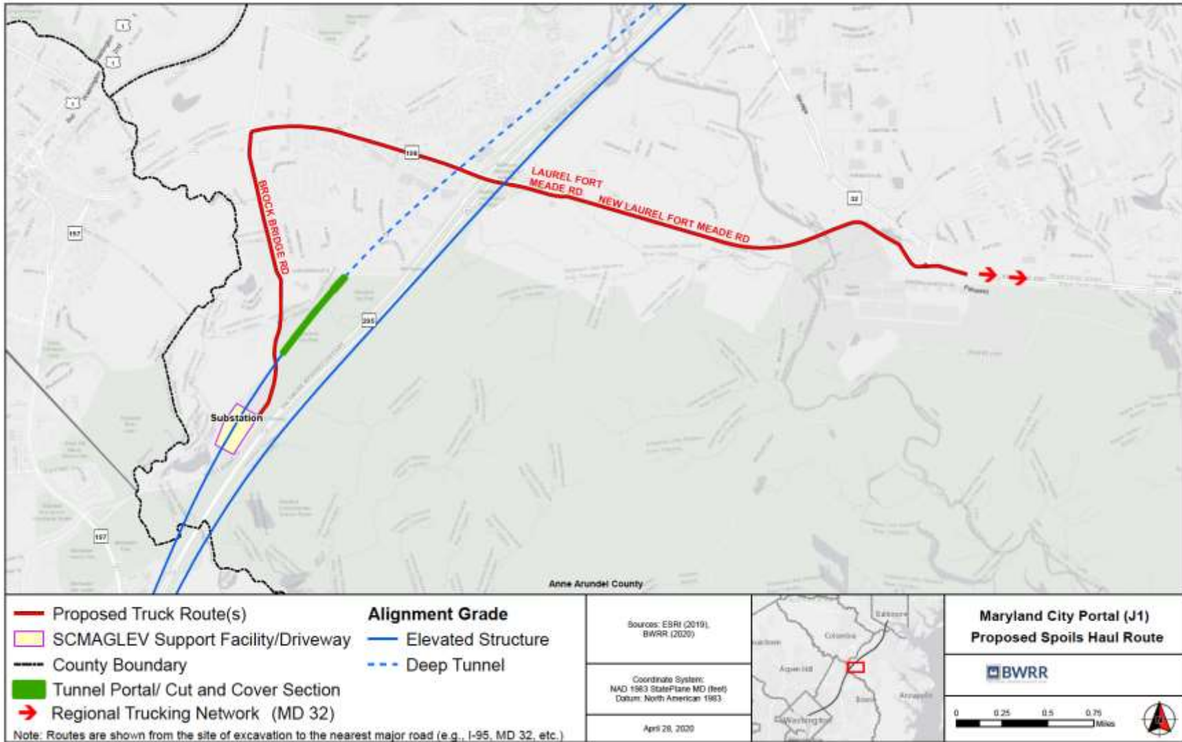
Figure 29. Proposed Haul Route for Maryland City Portal (Alignment Alternative J1)
