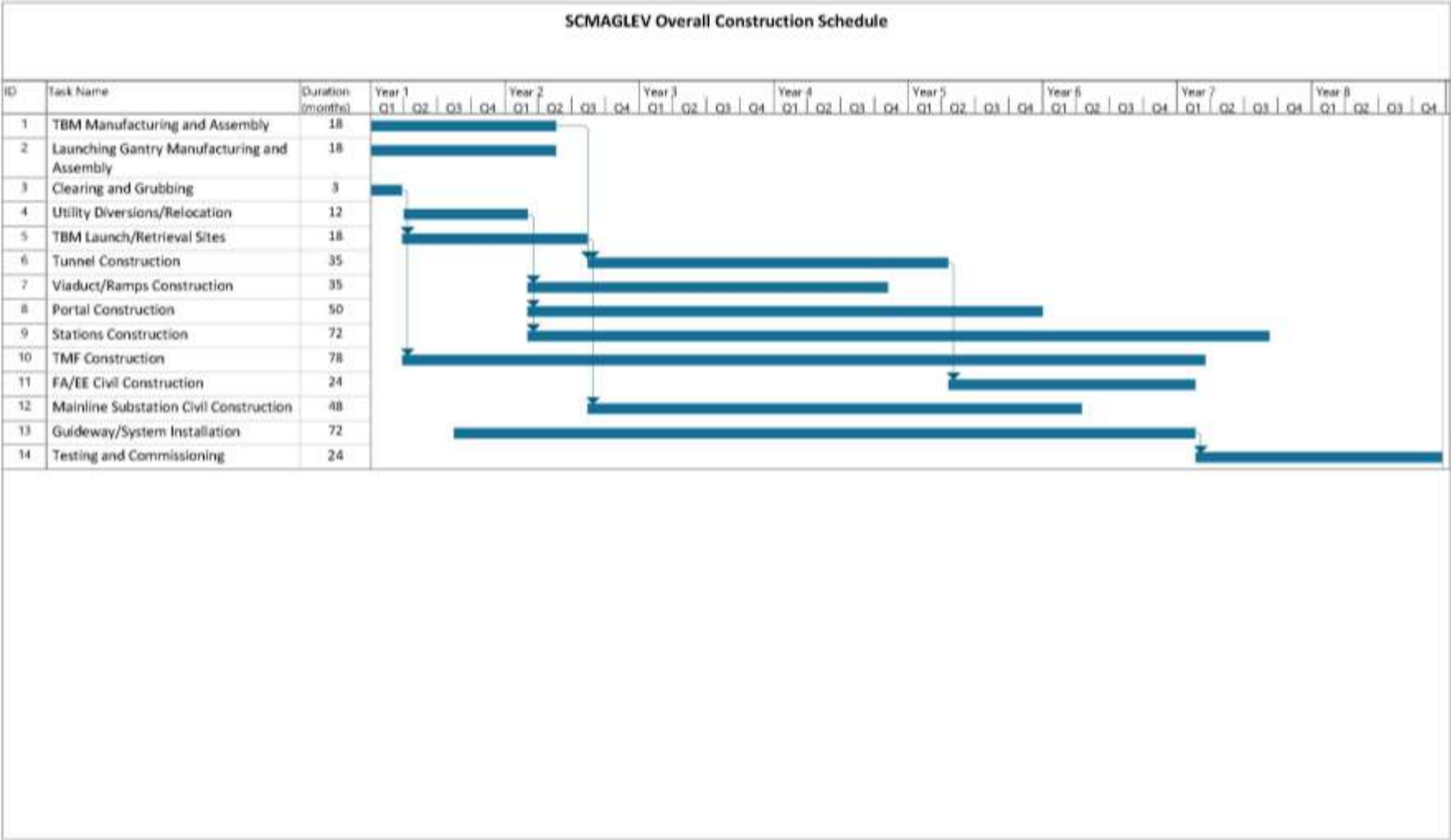
Figure 2. SCMAGLEV Overall Construction Schedule
