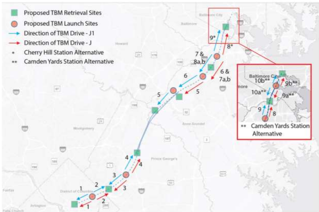
Figure 12. Proposed TBM Drives with Launch/Retrieval Sites
