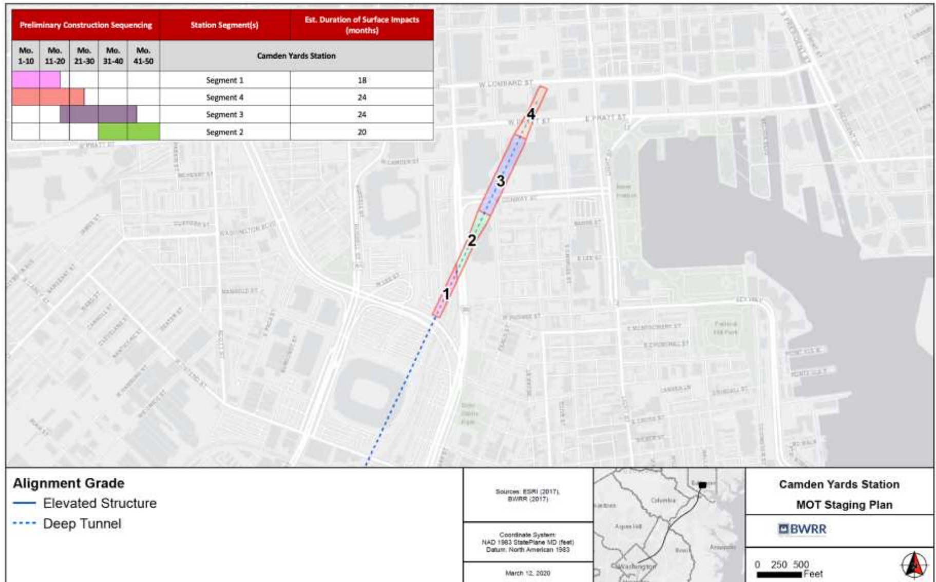
Figure 23. Construction Staging Segments for Camden Yards Station Alternative
