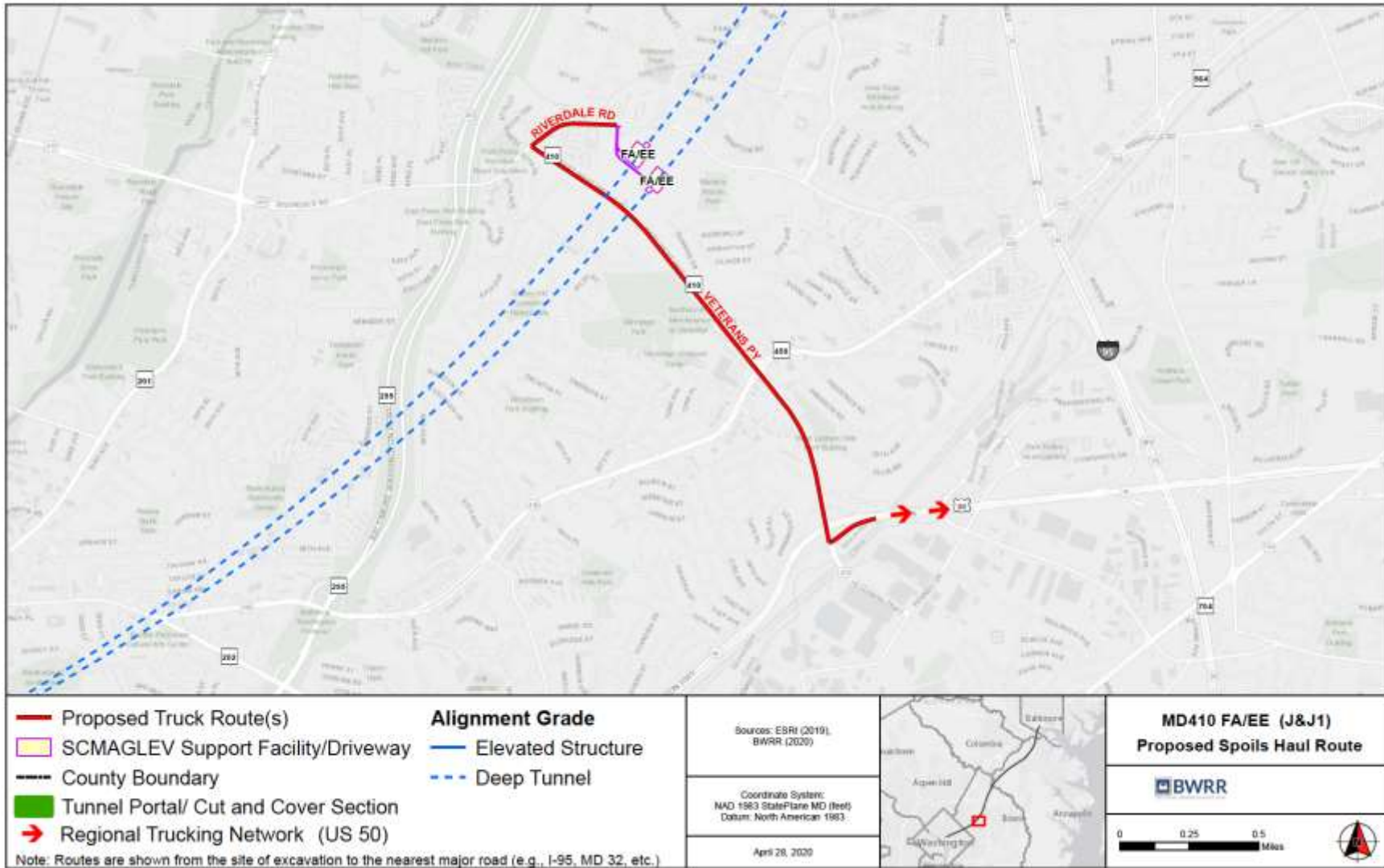
Figure 31. Proposed Haul Route for MD-410 FA/EE (Alignment Alternative J & J1)
