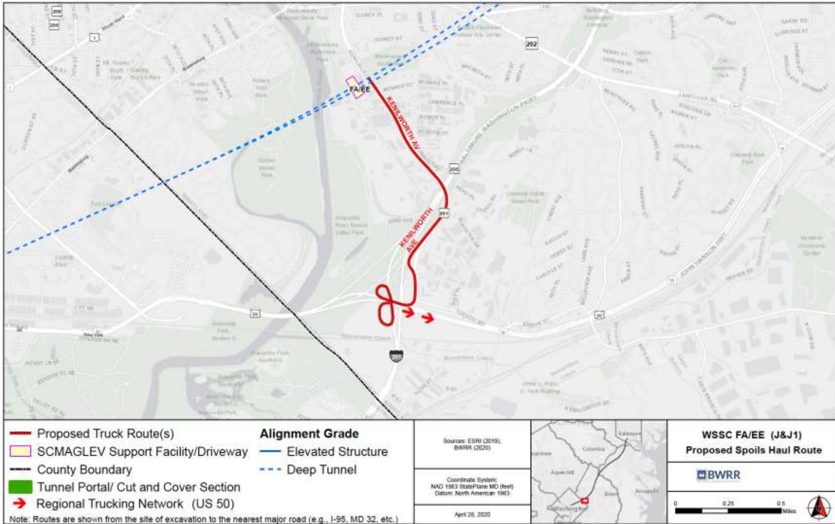
Figure 32. Proposed Haul Route for WSSC FA/EE (Alignment Alternative J & J1)
