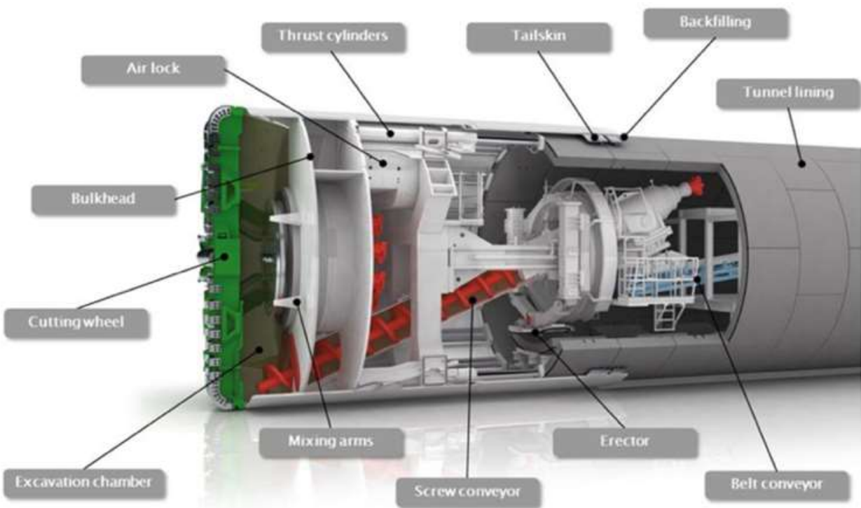
Figure 3. Schematic of EPB TBM (Courtesy of Herrenknecht)
