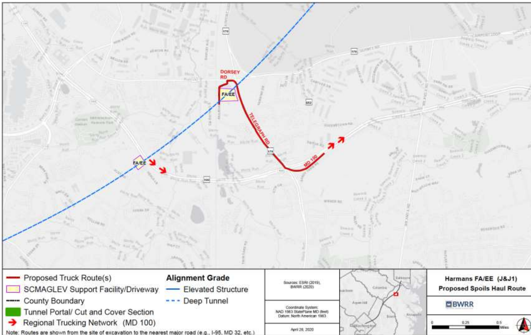
Figure 27. Proposed Haul Route for Harmans FA/EE (Alignment Alternative J & J1)
