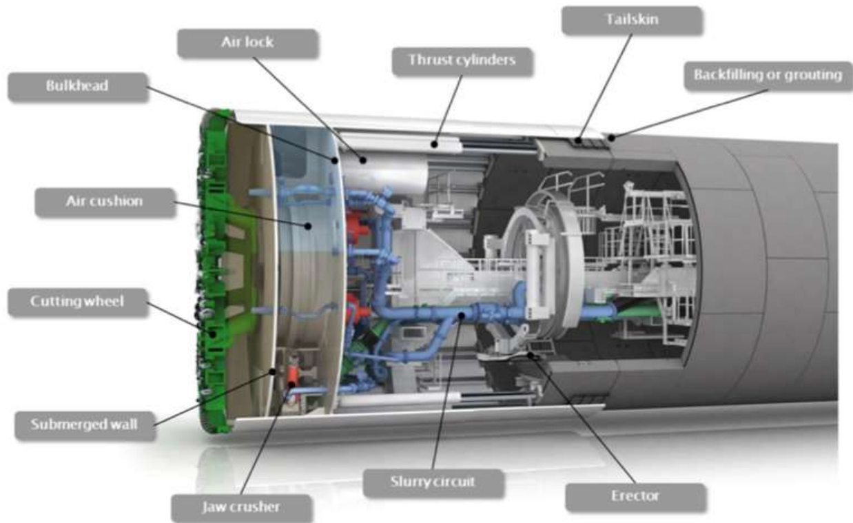
Figure 4. Schematic of SLURRY TBM (Courtesy of Herrenknecht)
